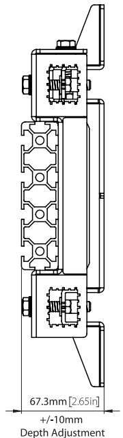
SIDE VIEW with BT8390 RAIL (Centre depth)
