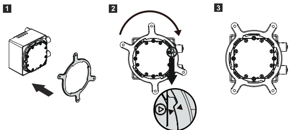
AMD Pump Clip
