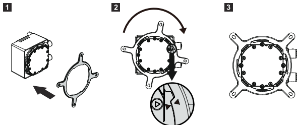
Intel Pump Clip
