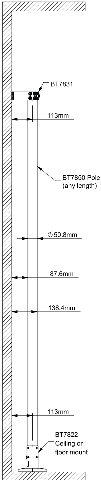
Floor-to-wall mounting position
