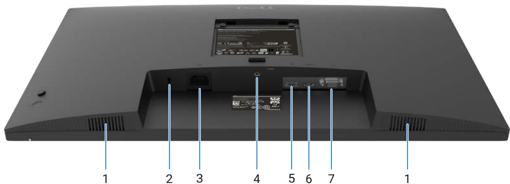
Figure 4. Bottom view
