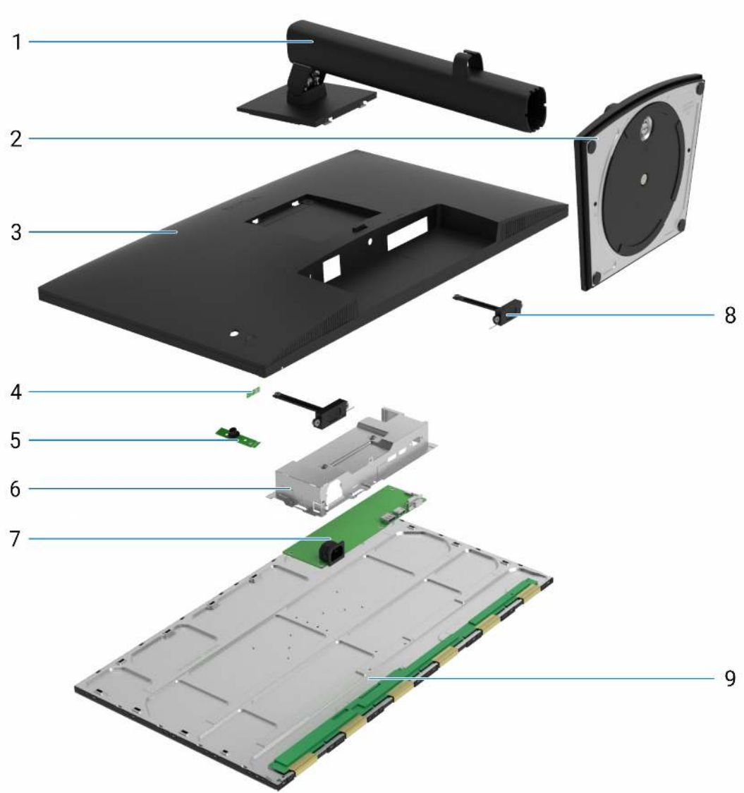
Figure 5. Major Components of E2726HS monitor
