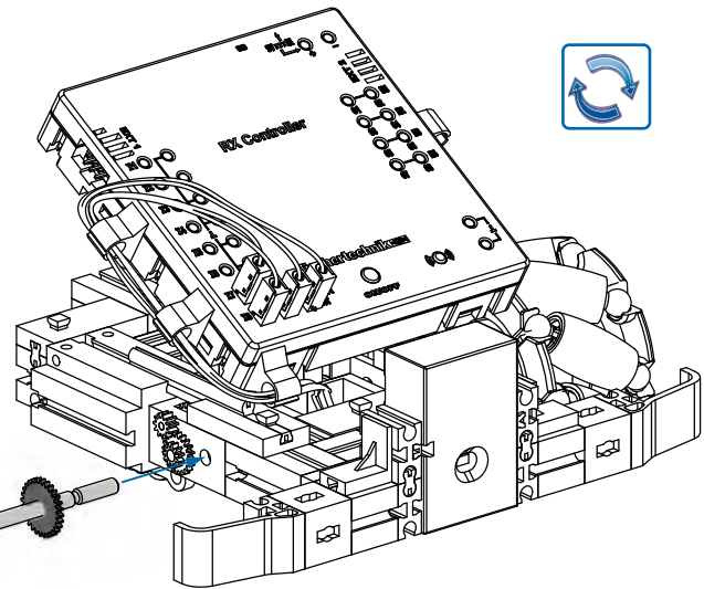
Omniwheel B
