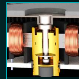
Fluid Dynamic Bearing
