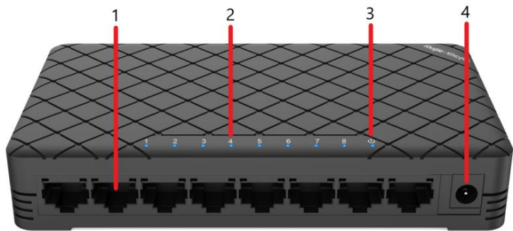
Figure 1-8 Figure 1-9 Front Panel of RG-ES08G
