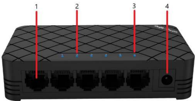
Figure 1-2 Figure 1-2 Front Panel of RG-ES05
