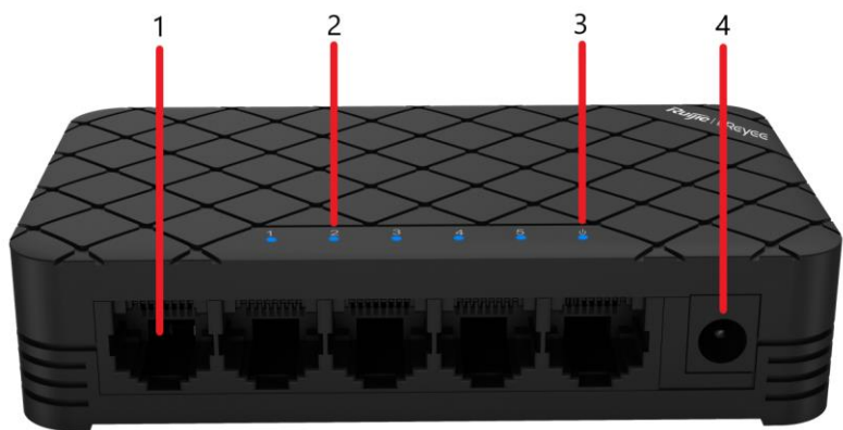
Figure 1-6 Figure 1-6 Front Panel of RG-ES05G
