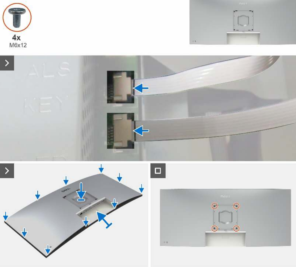
Figure 18. Installing the back cover
