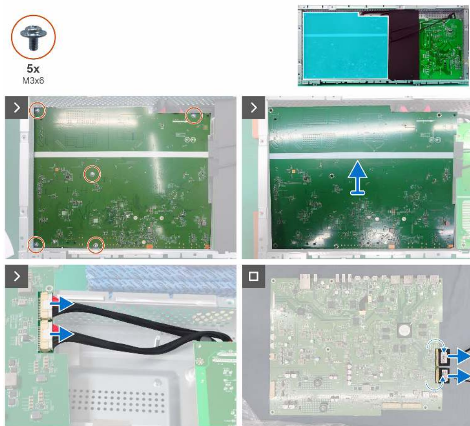
Figure 37. Removing the main board
