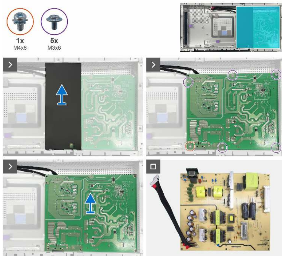
Figure 39. Removing the power board
