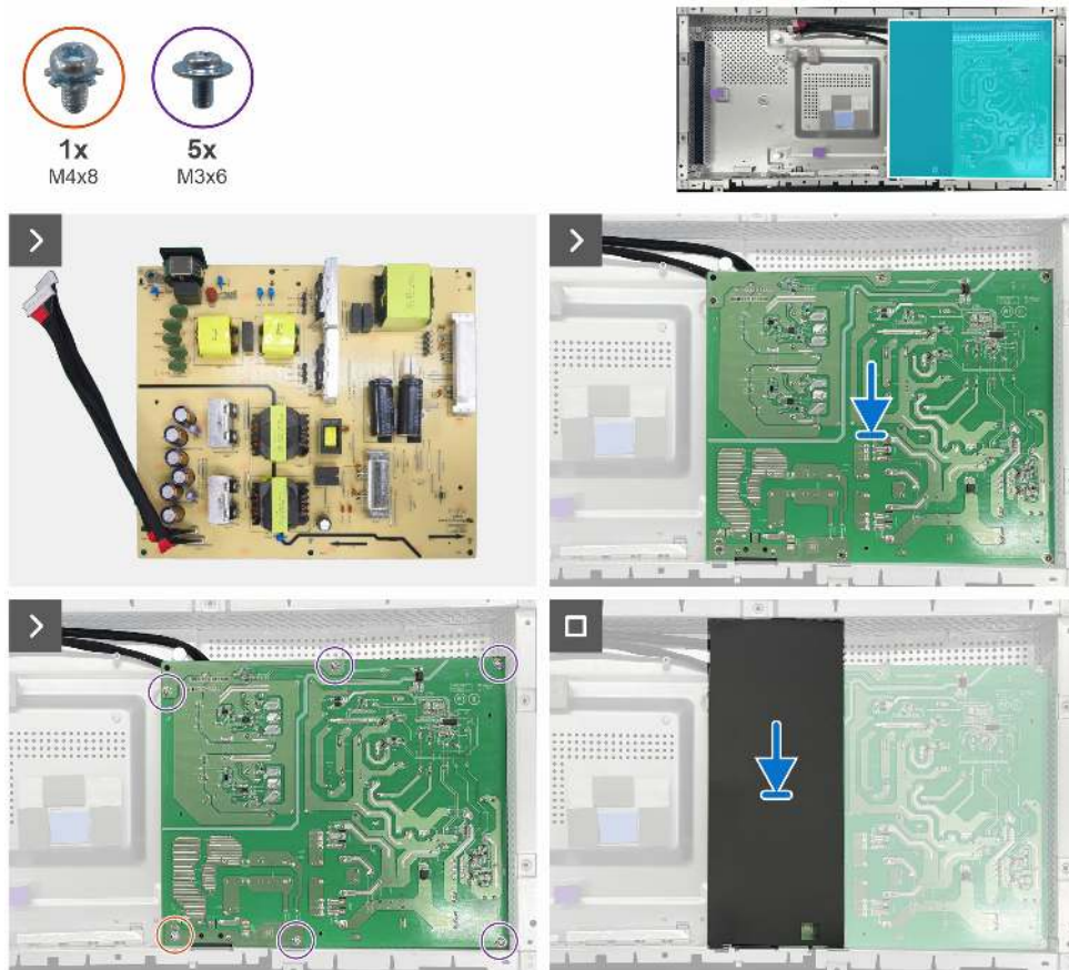
Figure 40. Installing the power board
