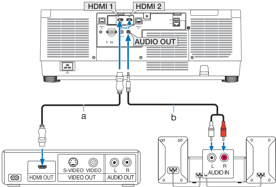
a: HDMI cable (not supplied) (Use a Premium High Speed HDMI Cable.) / b: Audio cable (not supplied)
