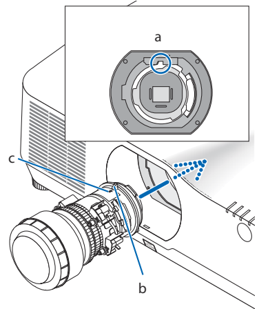
a: Guiding notch / b: Protrusion / c: Arrow
