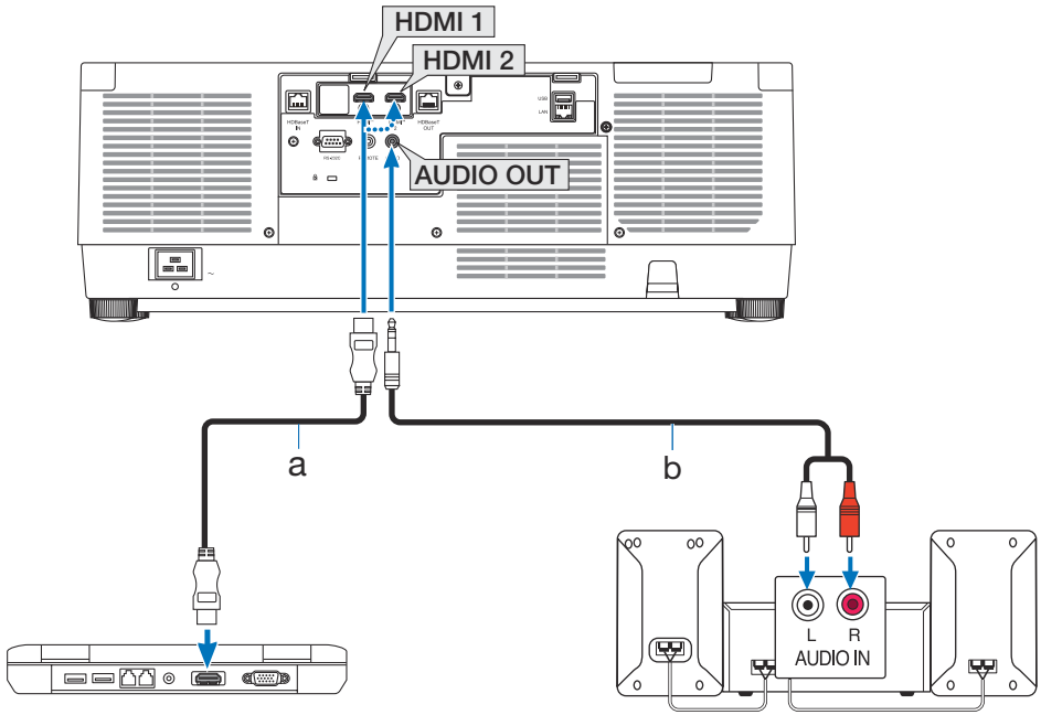
a: HDMI cable (not supplied) / b: Audio cable (not supplied)
