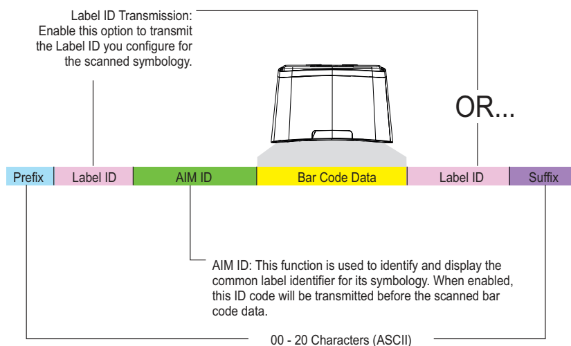
Figure 5. Breakdown of a Message String
