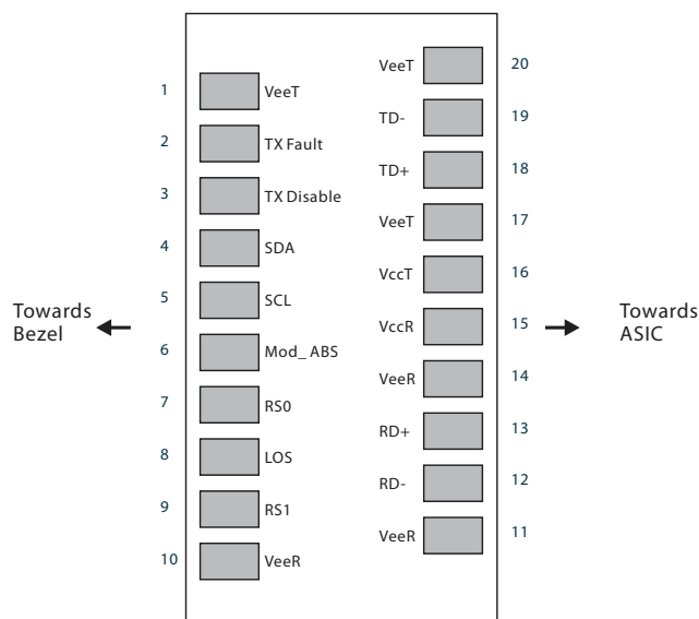
Pin-out of Connector Block on Host Board
