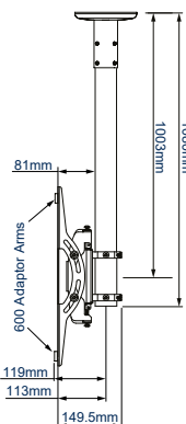
BT8424-100 SIDE VIEW - NO TILT
