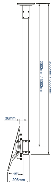
BT8424-200/300 SIDE VIEW - TILT UP
