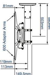
BT8424-050 SIDE VIEW - NO TILT
