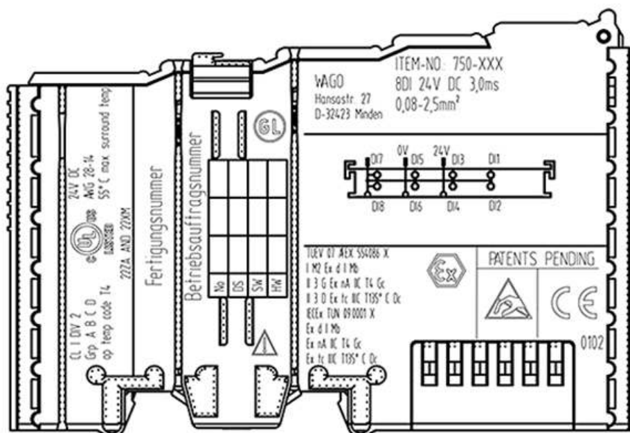
Figure 6: Side Marking Example for Approved I/O Modules According to ATEX and IECEx
