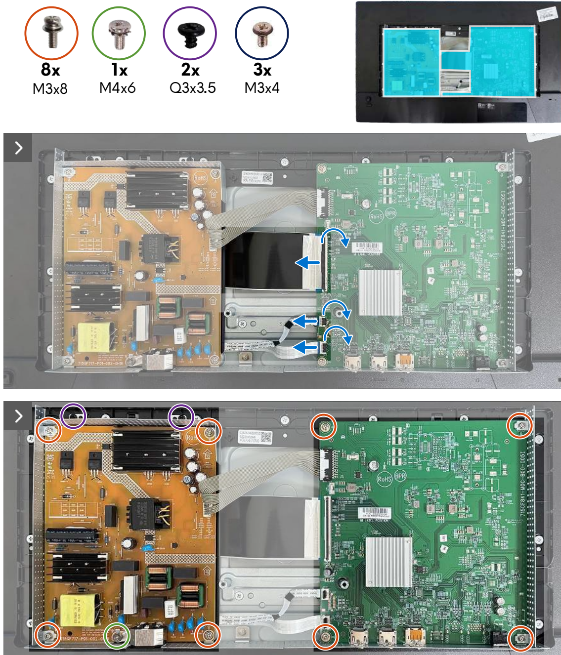
Figure 17. Removing the system board and power board
