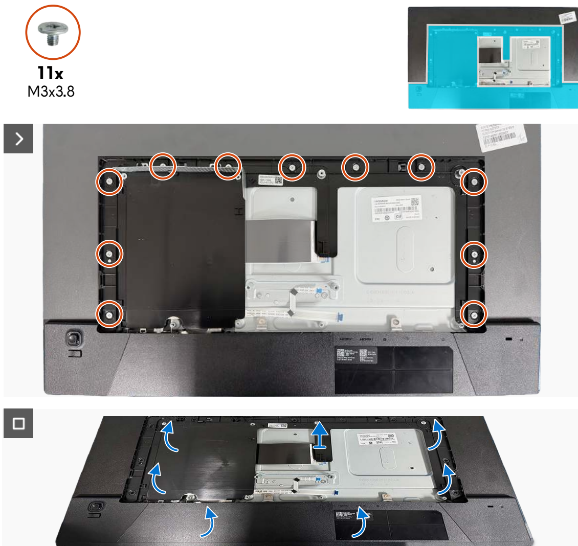
Figure 21. Removing the middle frame
