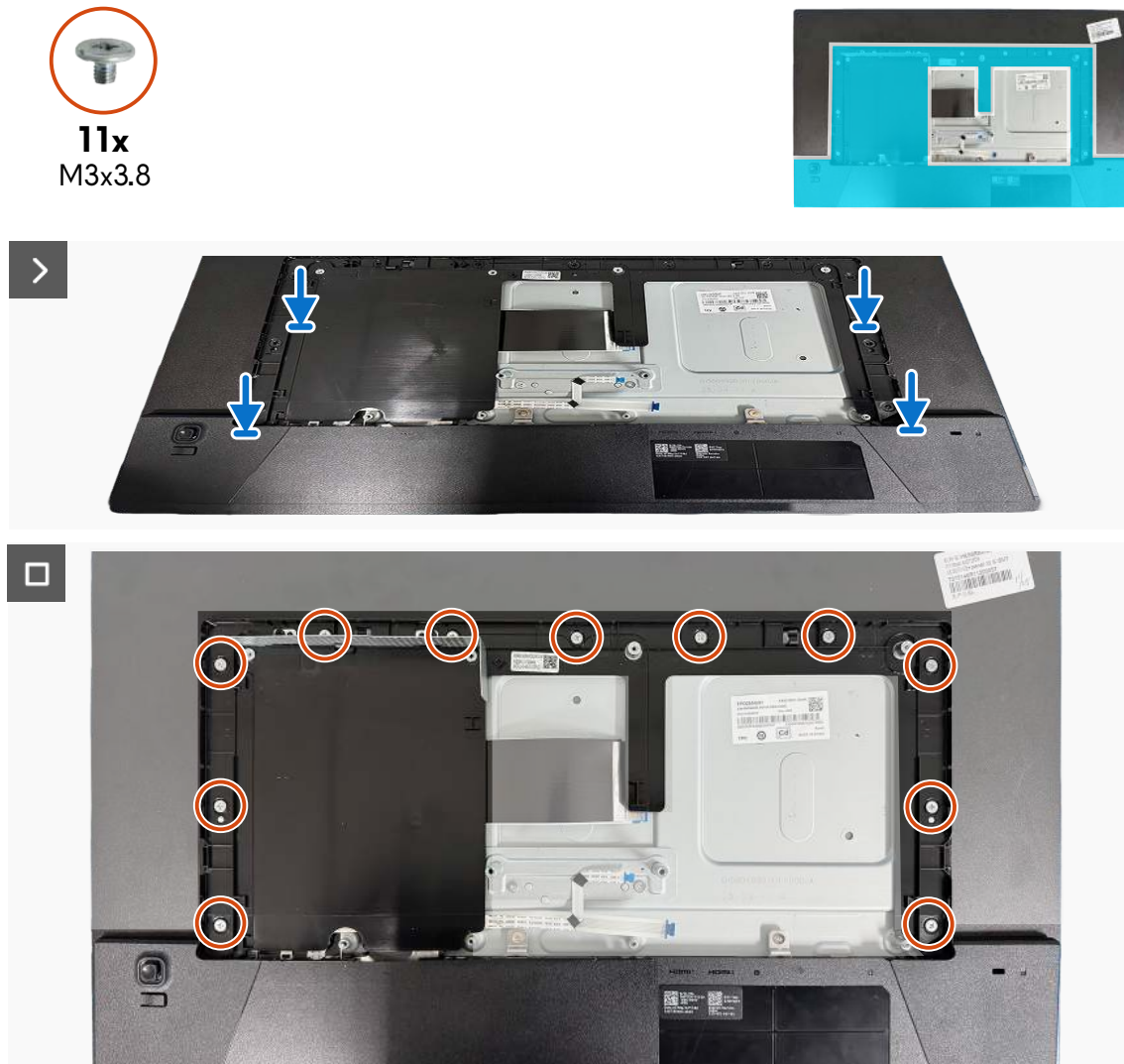
Figure 22. Installing the middle frame
