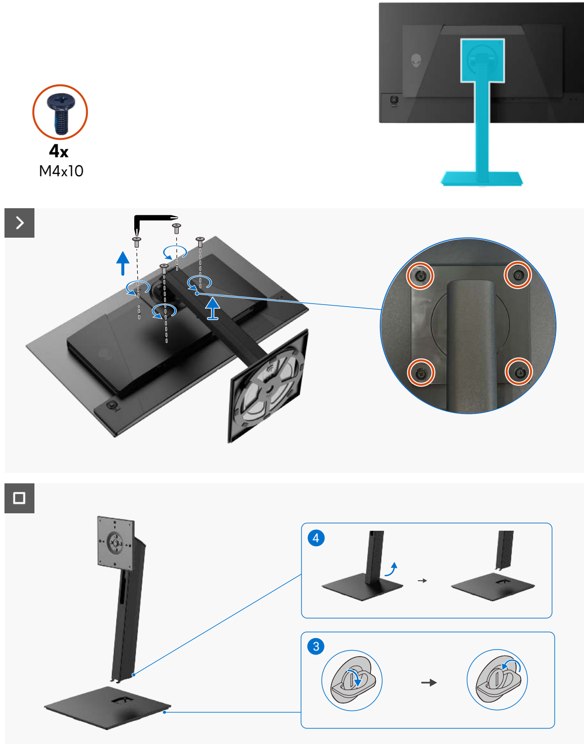
Figure 11. Removing the stand
