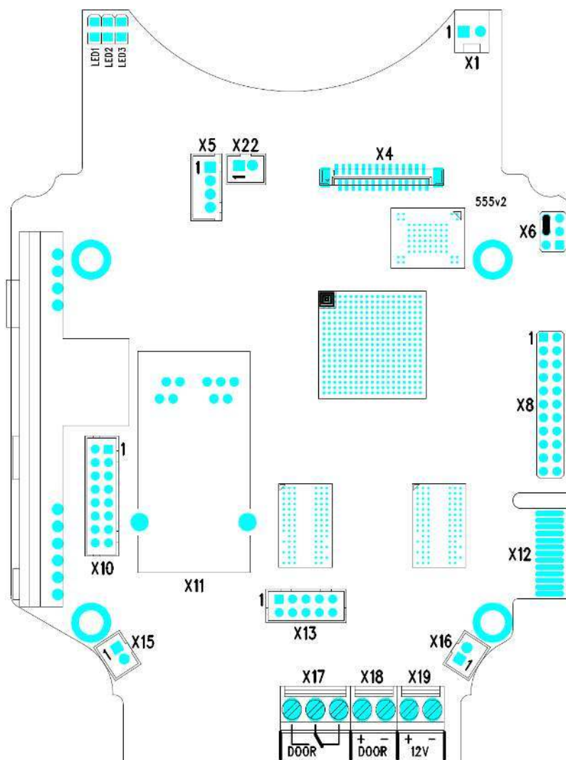
2N ® Helios IP Force Connectors, PCB Version 555v2
