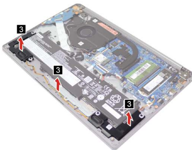
Figure 16. Remove speakers
