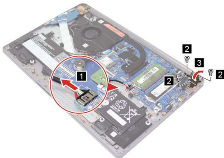
Figure 24. Disconnect cables
