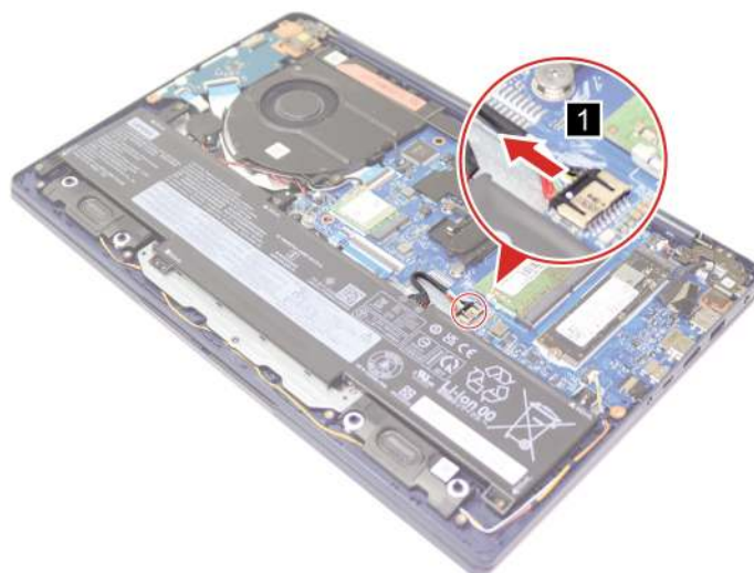
Figure 5. Disconnect the battery pack cable for 14-inch models
