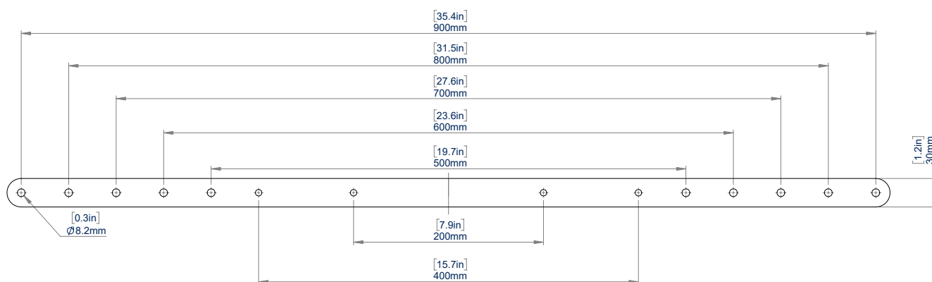
FRONT VIEW
