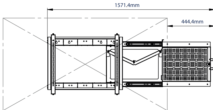
70" SCREEN - OPEN
