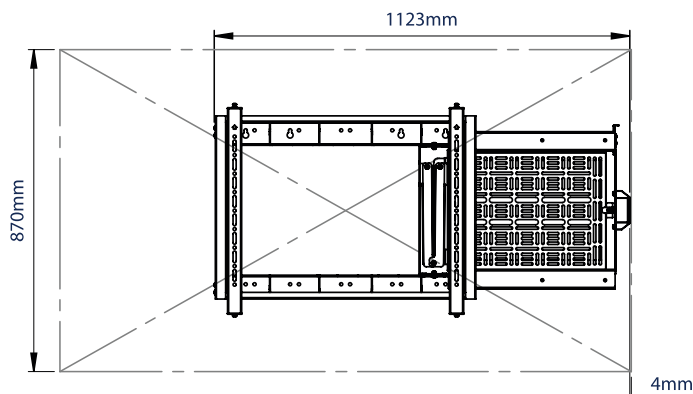
70" SCREEN - CLOSED
