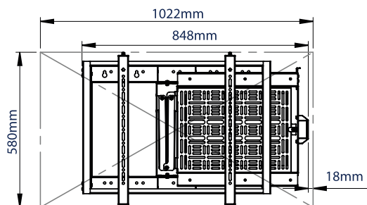
46" SCREEN - CLOSED
