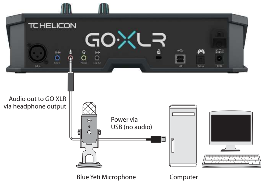
Blue Yeti Mic Recommended Connection
