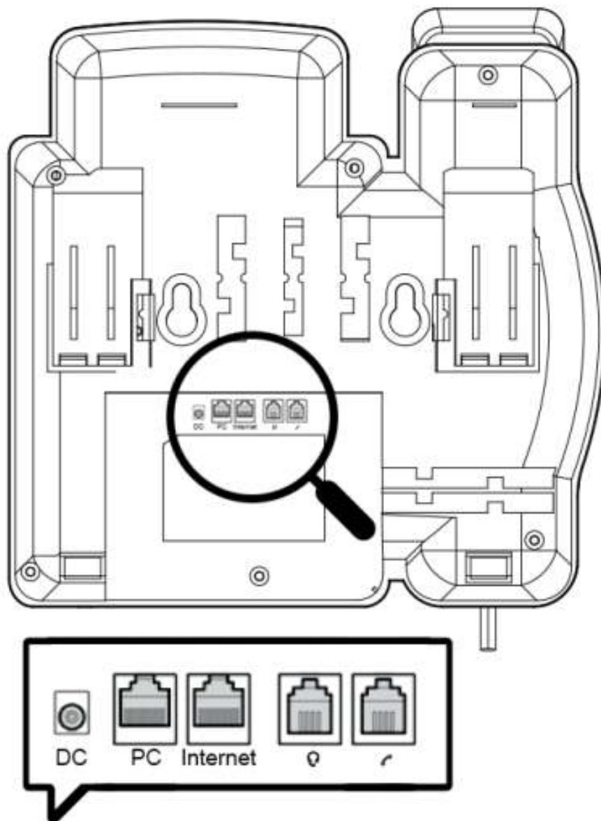
Figure 2-2: Rear View
