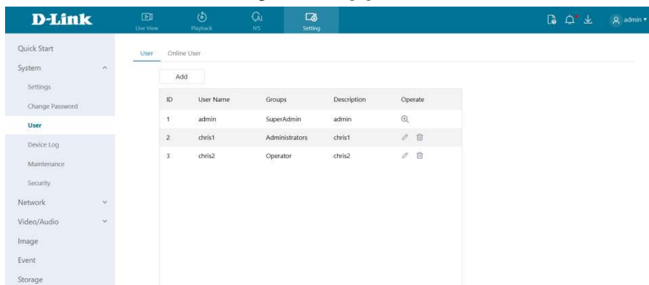
Figure 3-4 User page
