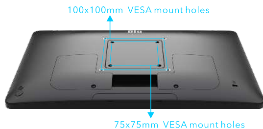
75x75mm VESA mount holes
