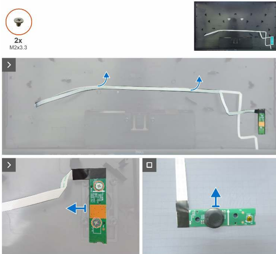
Figure 13. Removing the keypad board
