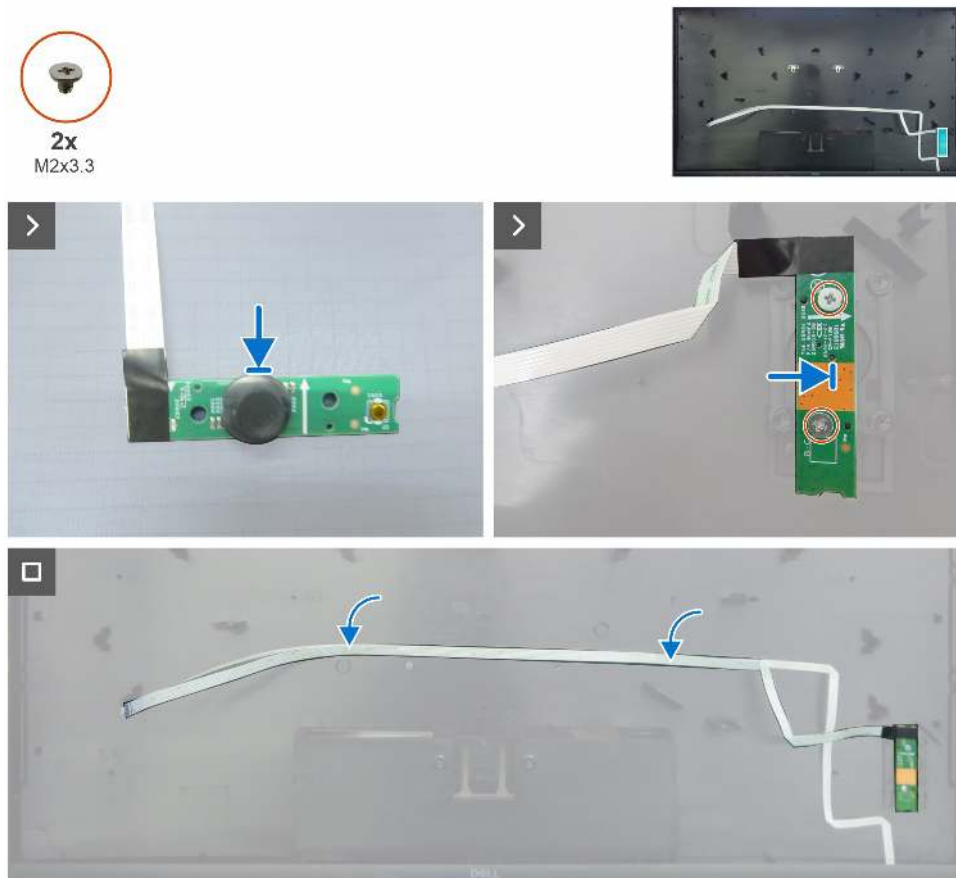
Figure 14. Installing the keypad board
