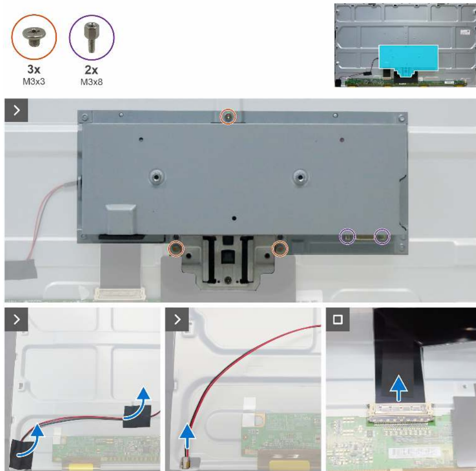
Figure 17. Removing the main chassis
