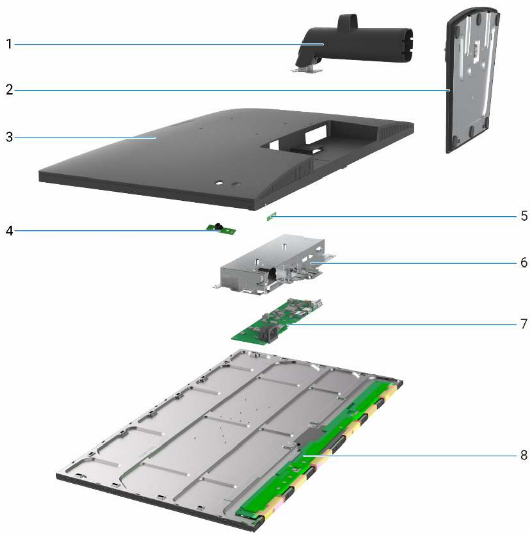
Figure 5. Major Components of E2726H monitor
