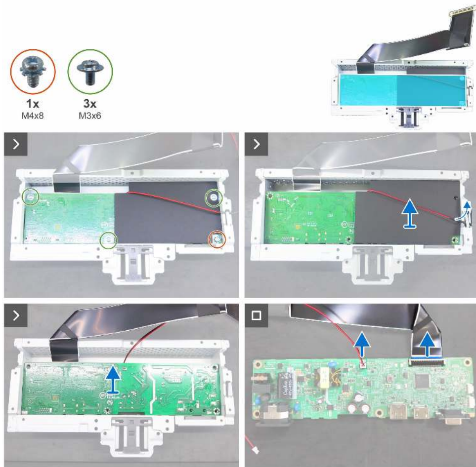
Figure 19. Removing the main board
