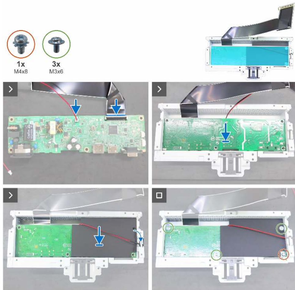
Figure 20. Installing the main board
