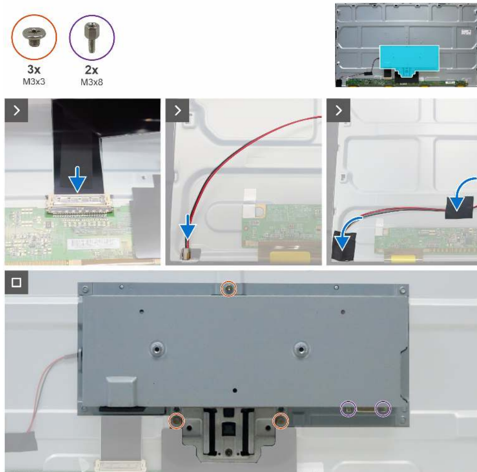
Figure 18. Installing the main chassis
