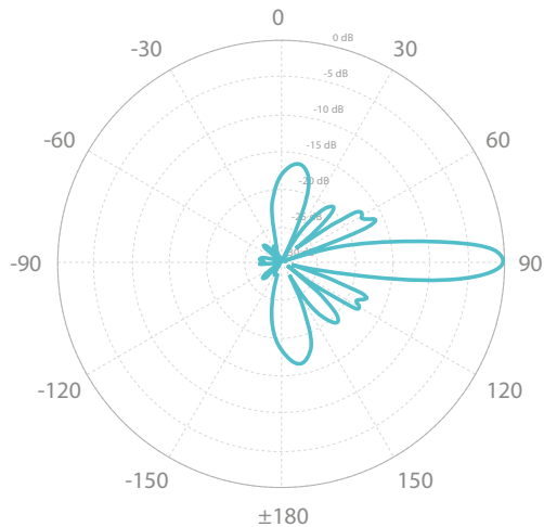
Vertical Elevation
