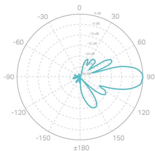
Horizontal Elevation
