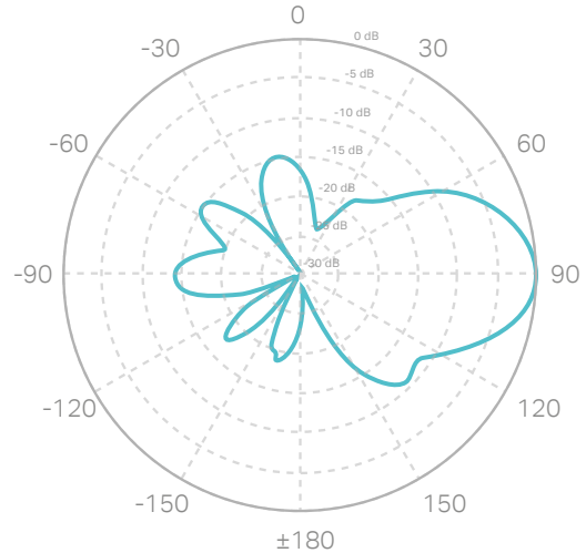
Horizontal Elevation
