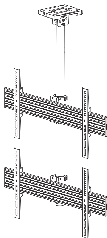
Fixed arms
