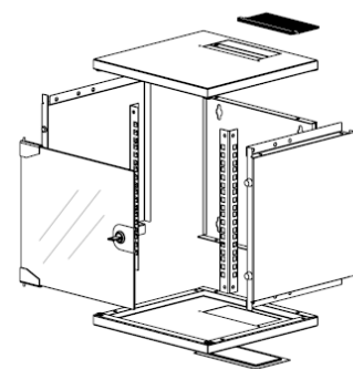
EXPLODED VIEW
