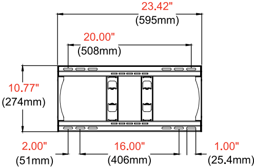
WALL PLATE DETAIL
