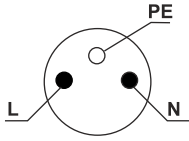
Power socket pin configuration
