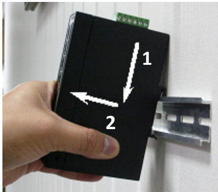
Figure 7: Remove Industrial Equipment in DIN-Rail mount.
