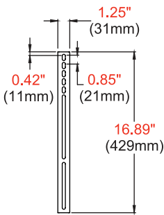
VERTICAL ADAPTOR
