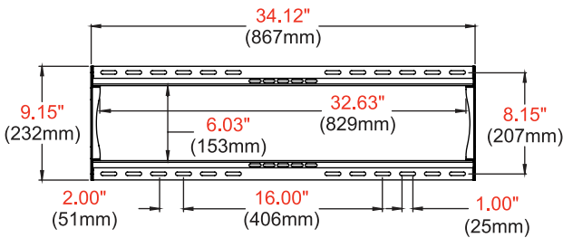
WALL PLATE
