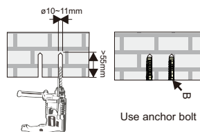
Concrete Ceiling mounting
