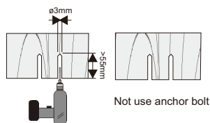
Dry- Ceiling mounting
