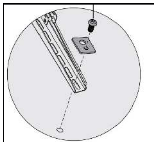
Securing the Vertical Bracket
