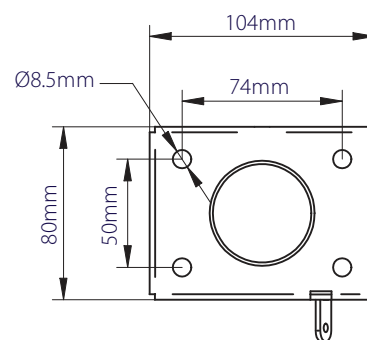
CEILING PLATE
