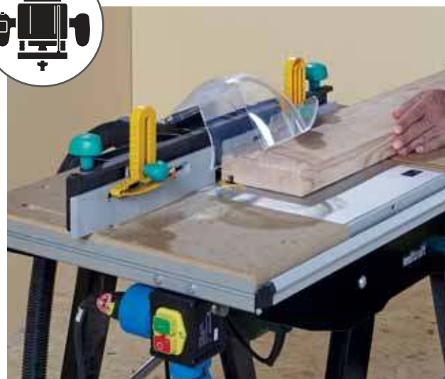
Milling table
