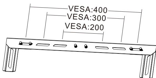
M Universal Soundbar Mount Small
