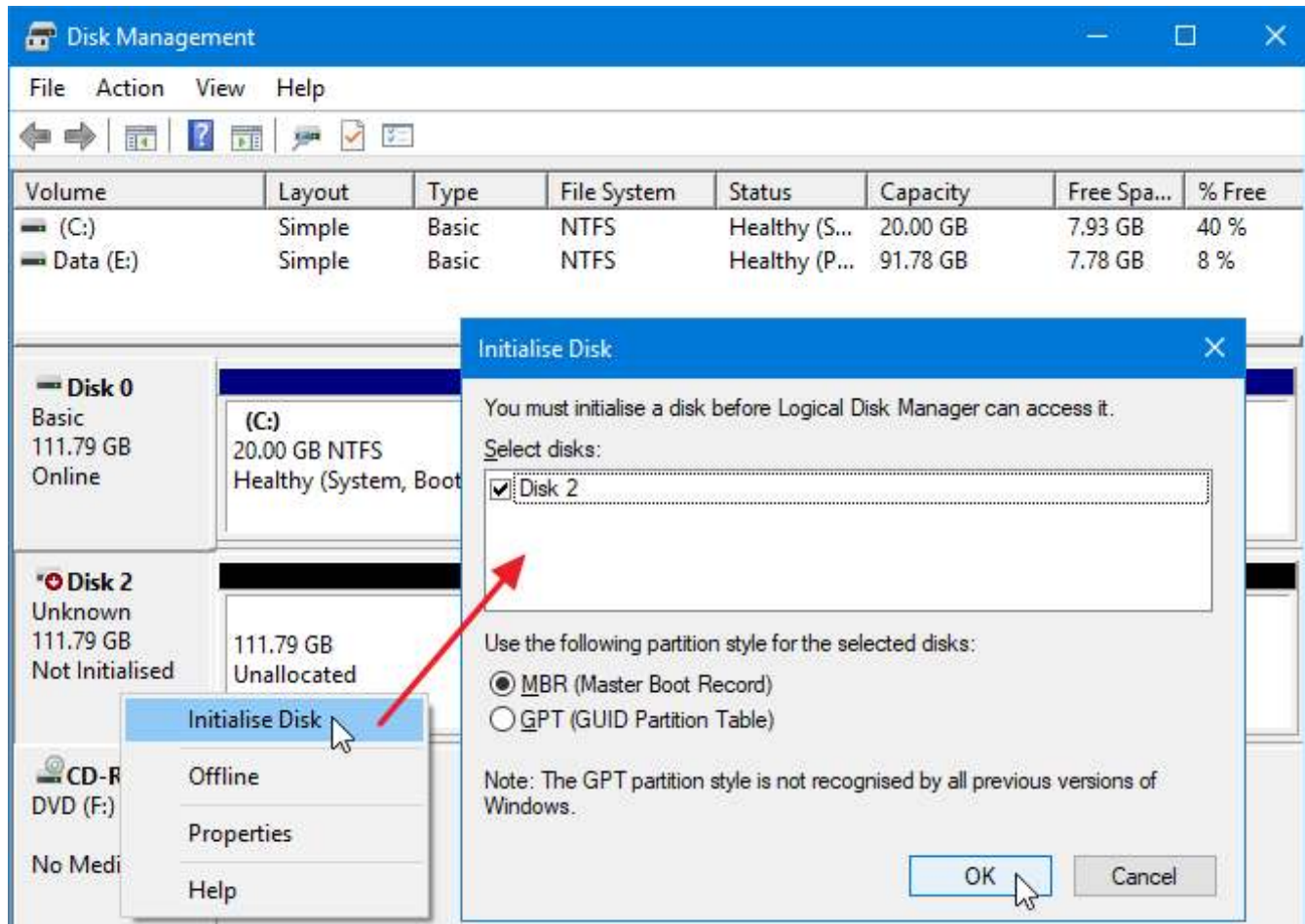
FIGURE 2. Disk initialization.
