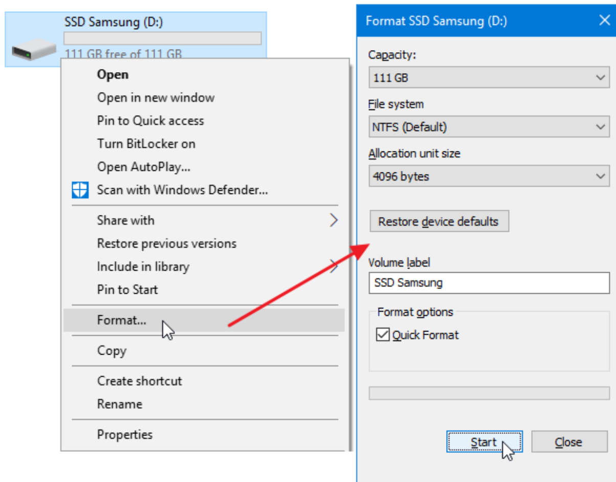
FIGURE 3. Disk formatting.
