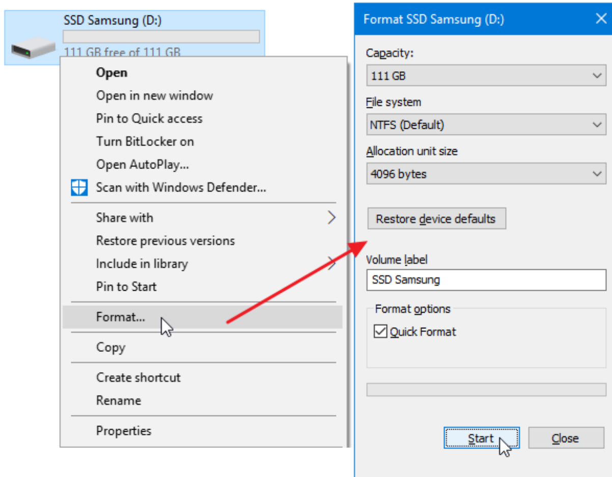
FIGURE 3. Disk formatting.
