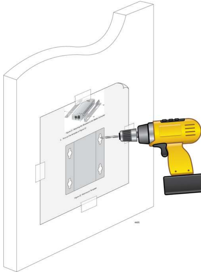
Figure 32. Placing the Template on the Wall
