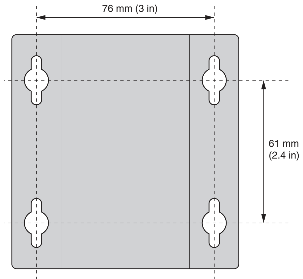
Figure 31. Wall-mount Template
