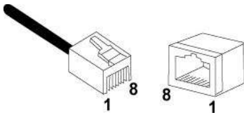
Figure 23. RJ45 Connector and Port Pin Layout
