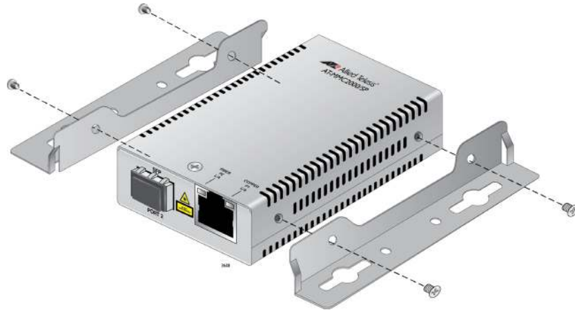
Figure 30. Attaching the Brackets to the Media Converter
