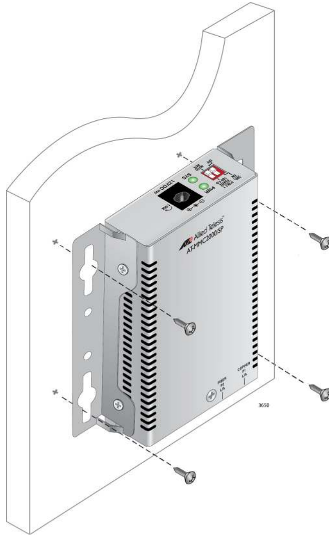
Figure 33. Securing the Media Converter to the Wall
