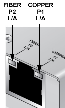
Figure 2. Port LEDs
