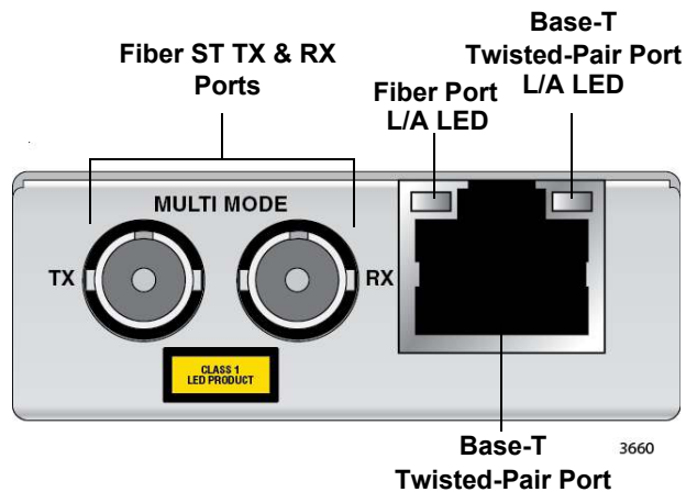
Figure 11. MMC2000/200/ST Series and AT-MMC200/LX/ST Front Panel
