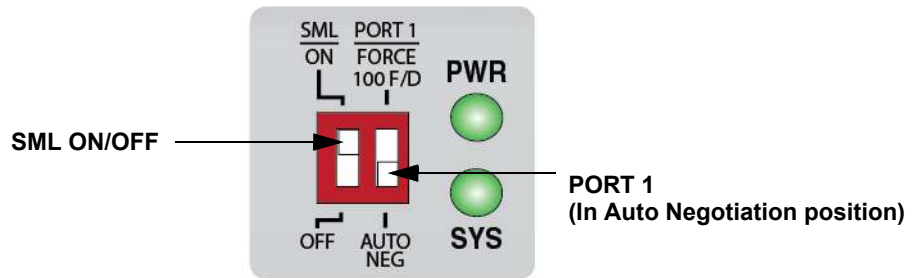
Figure 9. MMC2000/200 Series Converter Rear Panel DIP Switches
