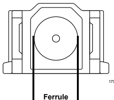
Figure 24. Ferrule in an SC Connector Plug
