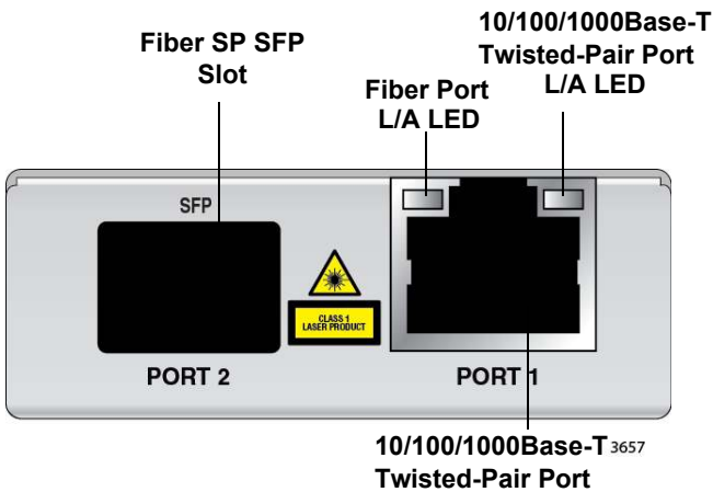
Figure 13. AT-MMC2000/SP Front Panel
