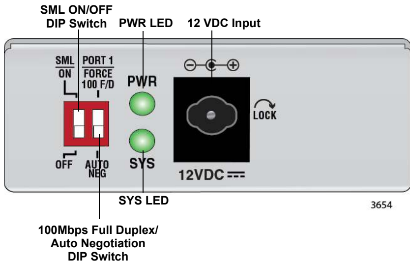
Figure 14. Media Converter Back Panel
