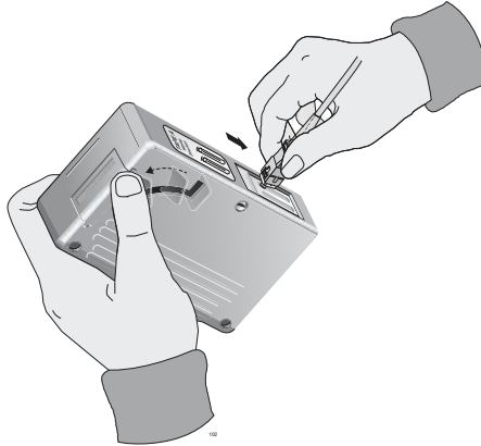
Figure 27. Rubbing the Ferrule Tip on the Cleaning Surface
