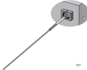
Figure 29. Cleaning a Recessed Ferrule
