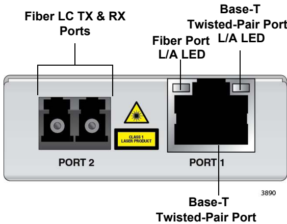
Figure 12. MMC2000/200LC Series and AT-MMC2000/LX/LC Front Panel
