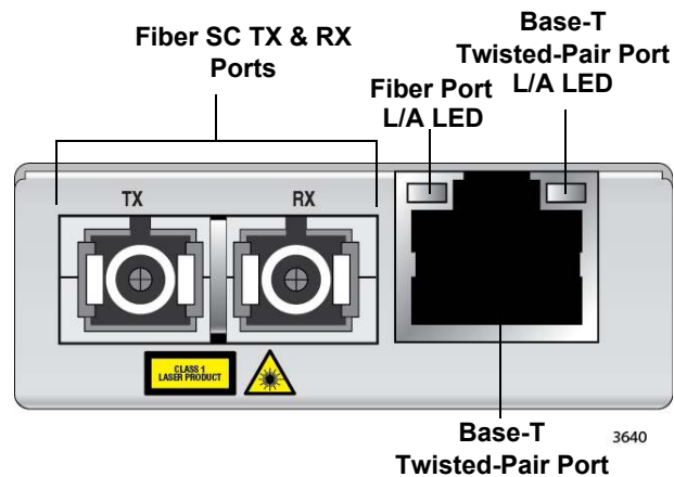
Figure 10. MMC2000/200/SC Series and MMC2000/200/LX/SC Series Front Panel
