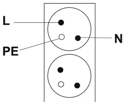
Gniazdo PN-E-93201
