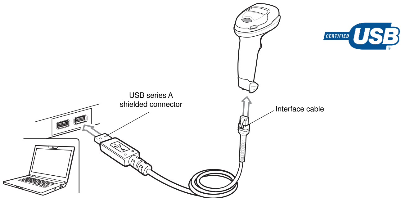
Figure 6-1 USB Connection.
