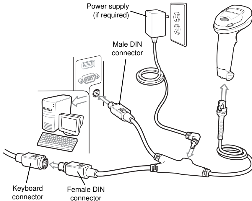
Figure 10-1 Keyboard Wedge Connection
