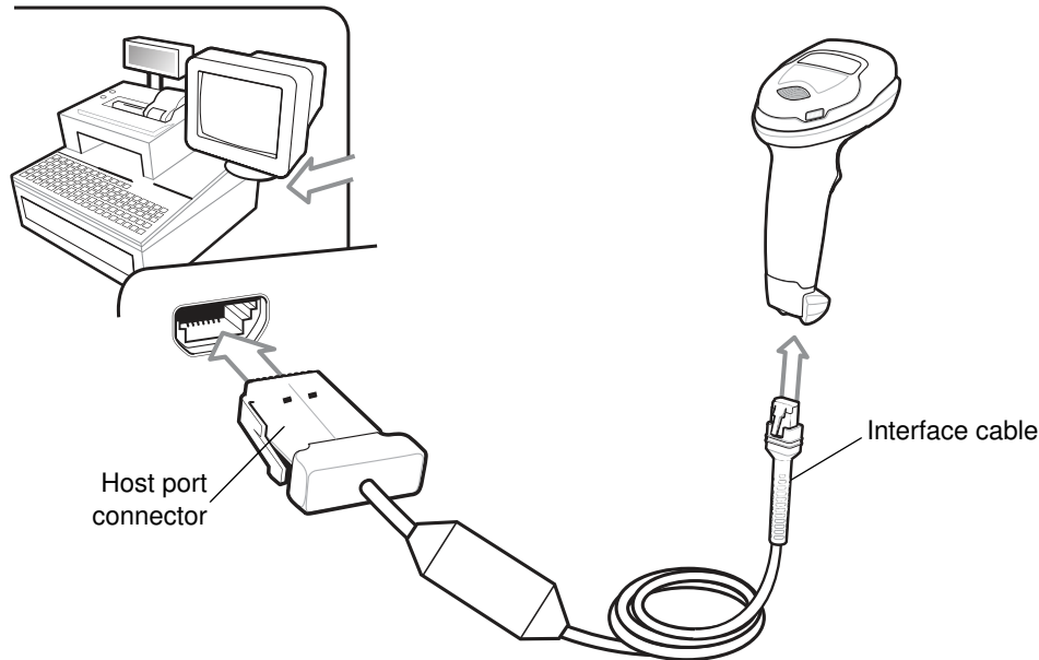
Figure 9-1 IBM Connection
