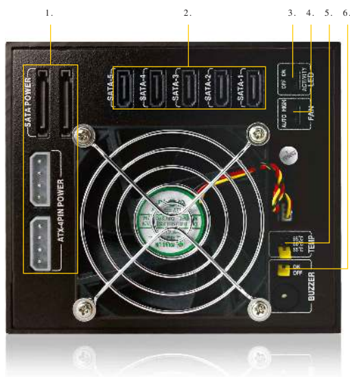
Rear view IB-565SSK
