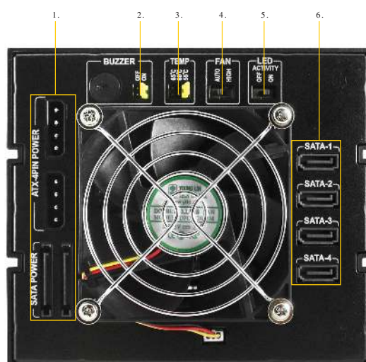
Rear view IB-563SSK
