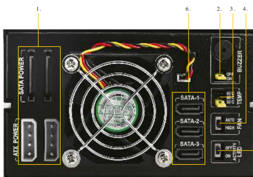
Rear view IB-563SSK
