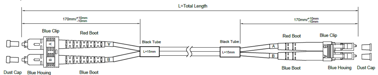
Example SM OS2 - SC to LC
