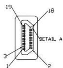
HDMI 19P MALE
