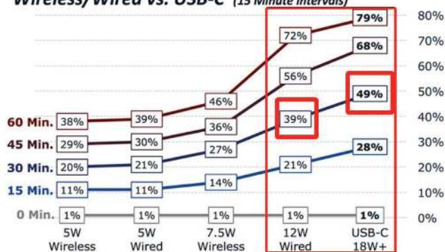
iPhone X Battery Percentage by Charging Method: Wireless/Wired vs. USB-C (15 Minute Intervals)
