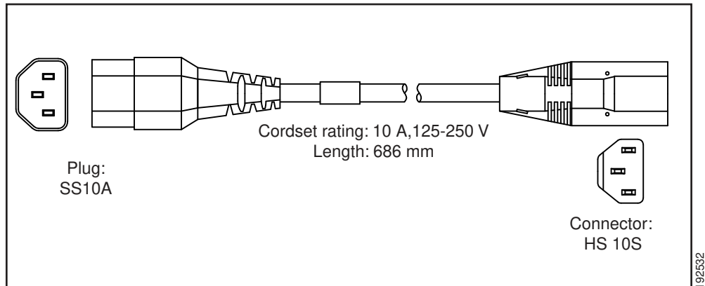
Figure C-15 CAB-C13-CBN
