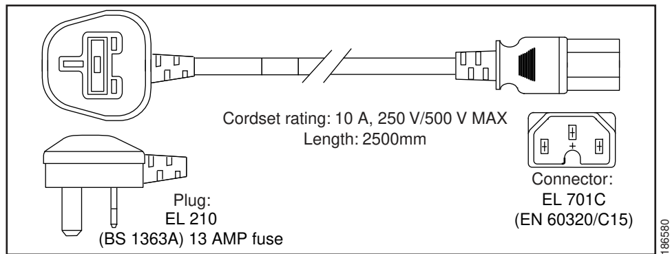
Figure C-9 CAB-9K10A-UK
