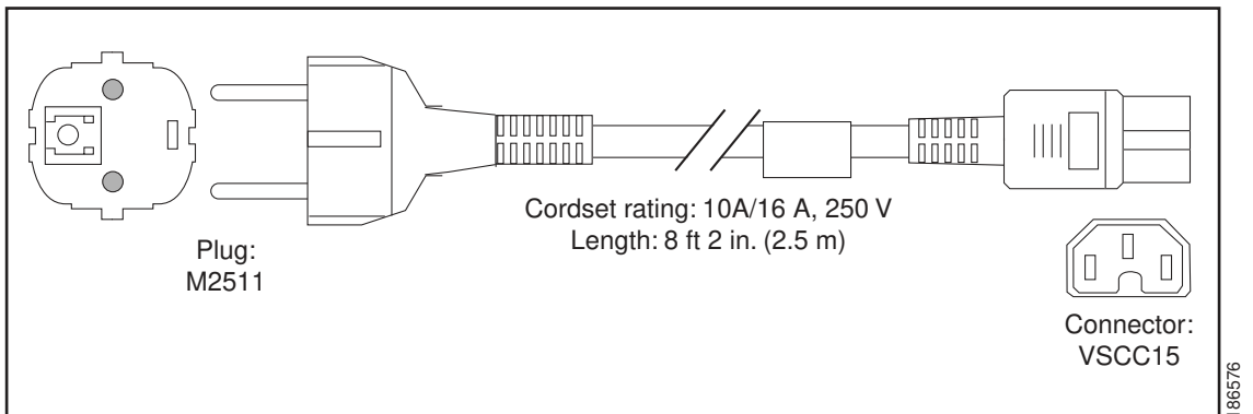
Figure C-4 CAB-9K10A-EU
