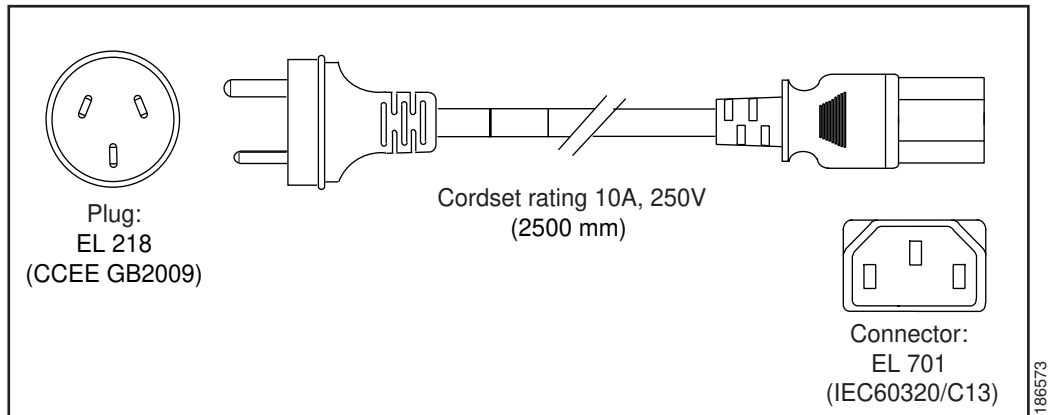
Figure C-3 SFS-250V-10A-CN
