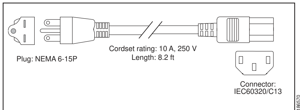
Figure C-11 CAB-N5K6A-NA
