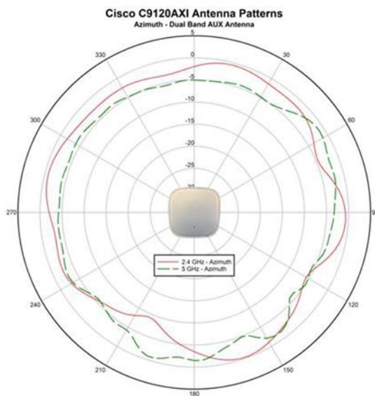
Azimuth
