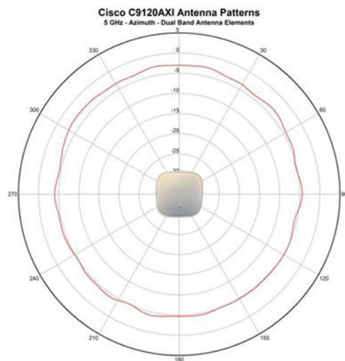
5 GHz Azimuth
