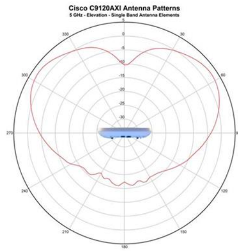
5 GHz Elevation
