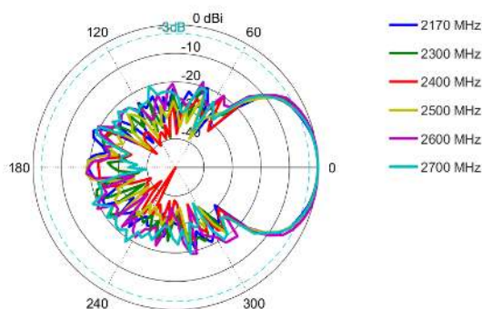
Elevation: 2170 – 2700 MHz
