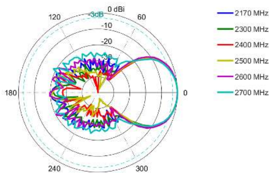
Azimuth: 2170 – 2700 MHz
