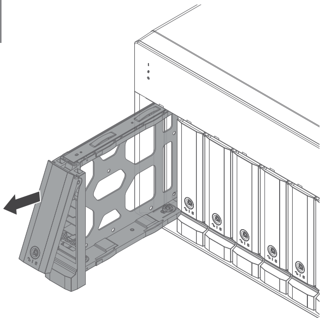
3.5-inch HDD
