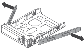
3.5-inch HDD
