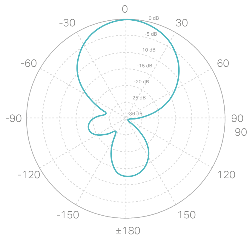
Horizontal Azimuth
