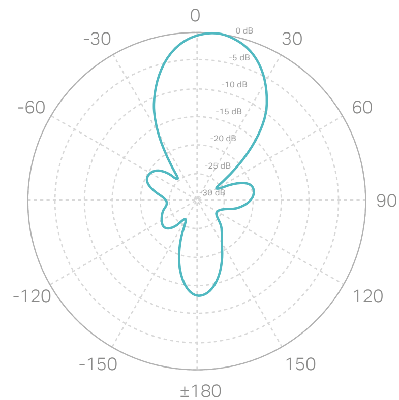
Horizontal Elevation
