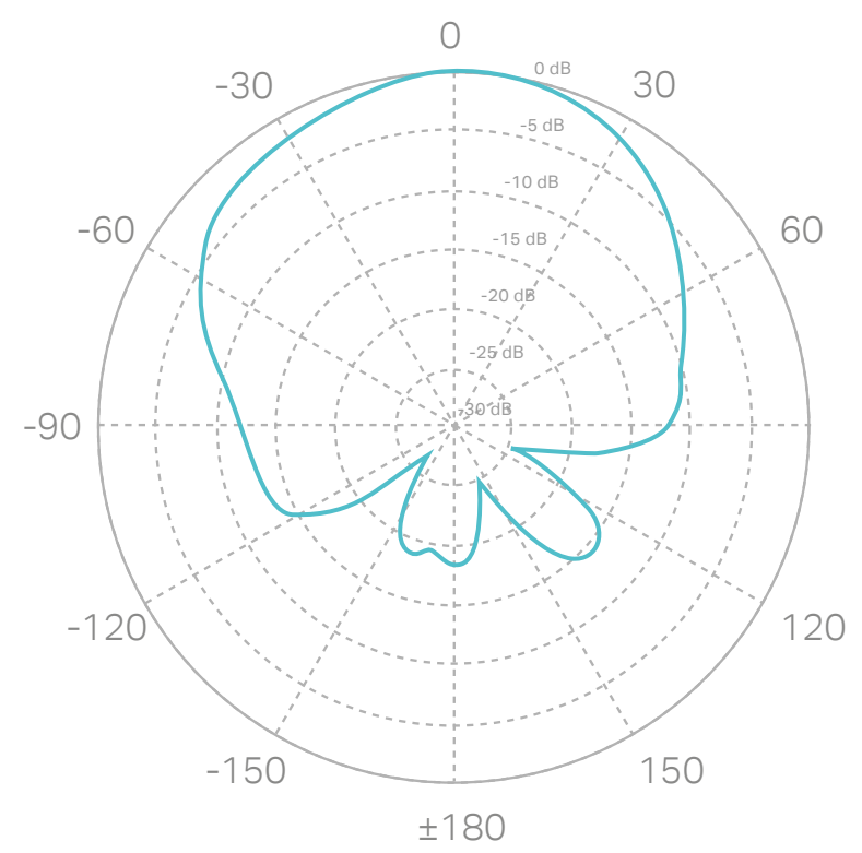
Horizontal Azimuth
